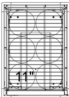
11" Covered Plate Configuration stacked four shelves 4 plates high.
